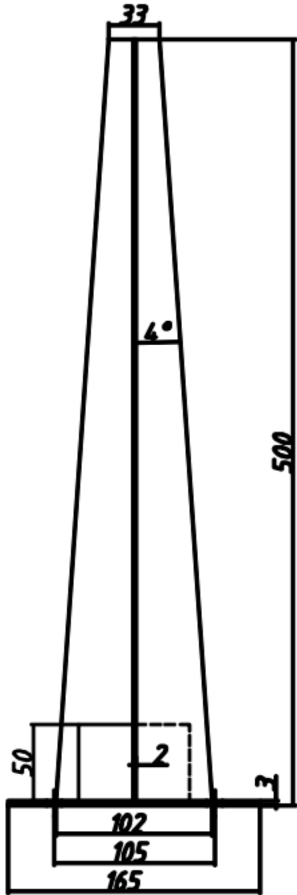
Mailbox Fork MB250 measured in centimeters
